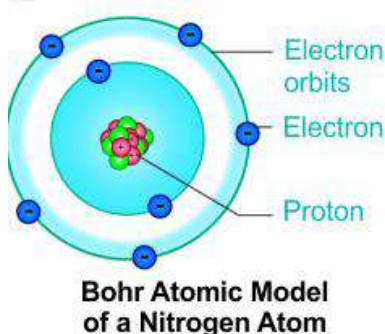
Figure 1.1: Atomic model of Bohr
