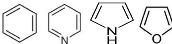
Pyridine
