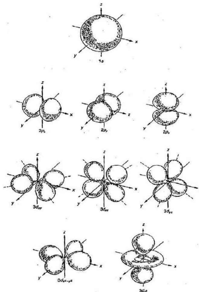
Fig 2.5: Angular distribution functions for various orbitals
