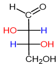
Threose
